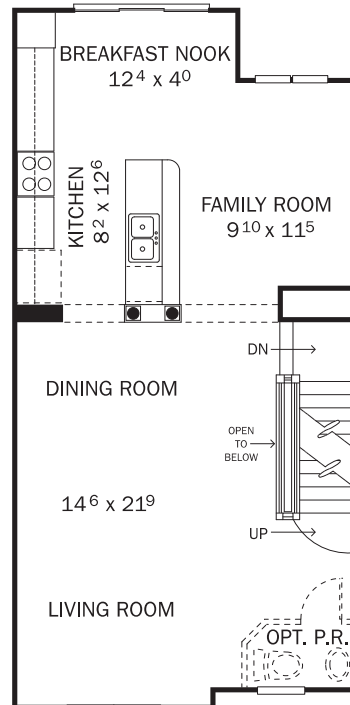
FIRST FLOOR (OPTIONAL 4' EXTENSION)
