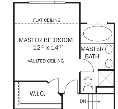
SECOND FLOOR (OPTIONAL 4' EXTENSION)
