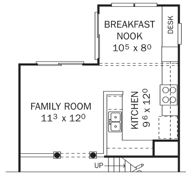
FIRST FLOOR (OPTIONAL 4' EXTENSION)
