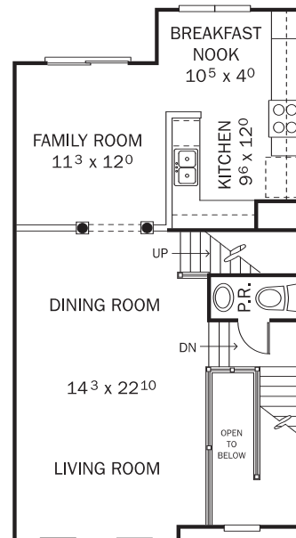
FIRST FLOOR (OPTIONAL 4' EXTENSION)
