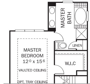
SECOND FLOOR (OPTIONAL 4' EXTENSION)
